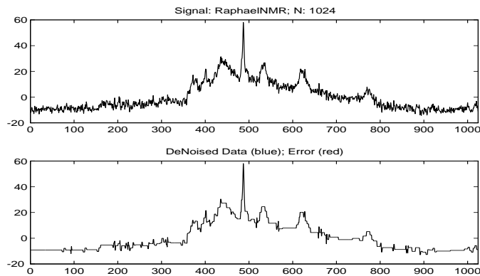
Figure 2: Denoising NMR Data
