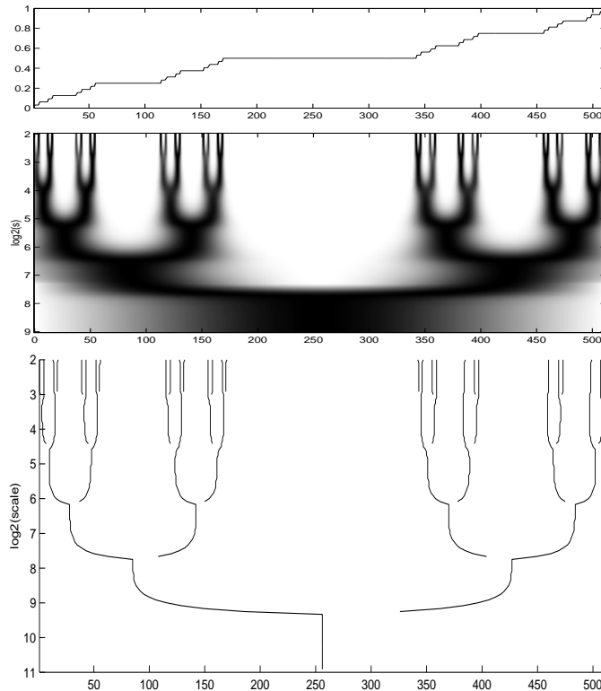
Figure 10: Devil's staircase and its wavelets transform
