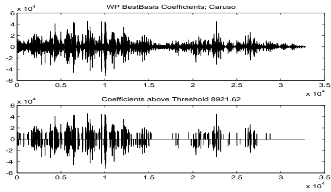
Figure 4: WP Coefficients, Caruso Signal
