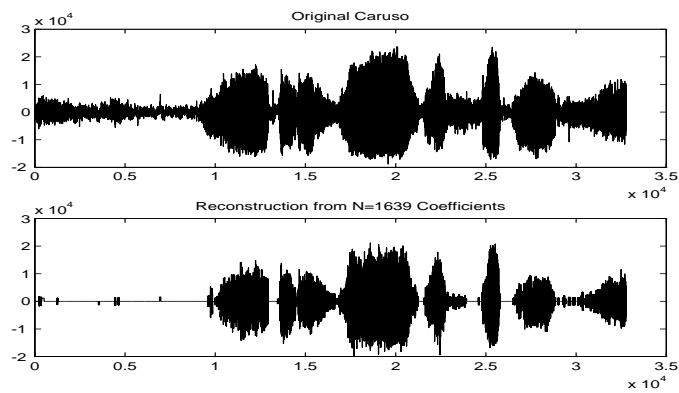
Figure 5: Denoised Caruso Signal
