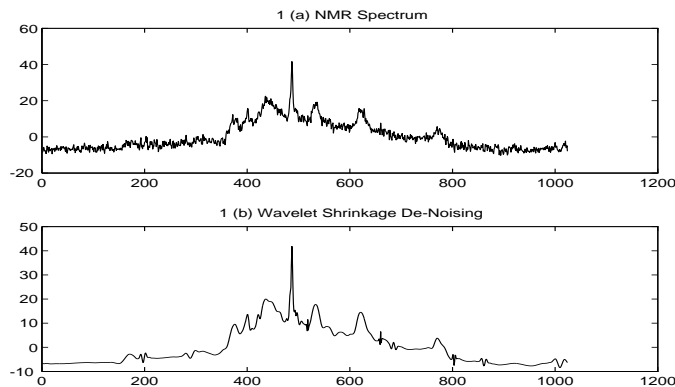
Figure 1: First Figure of Short Course
