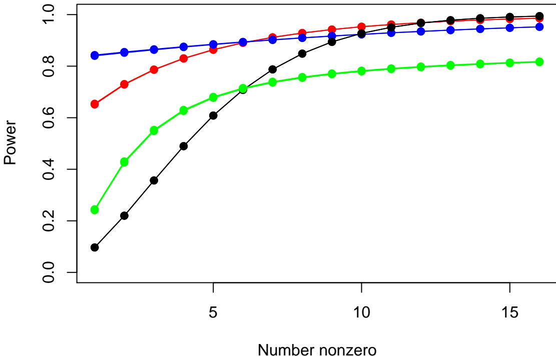
Top Fisher (red) Top LRT (blue) Top Stouffer (black) Stouffer (green) \alpha=.01 power=.8
