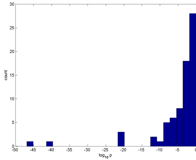
Figure 3. Histogram for p-values of information content NI_{seq} in flanking region of motifs discovered for yeast cell cycle. The flanking region of 20 bases (10 each on the left and right of the motif) is selected.
