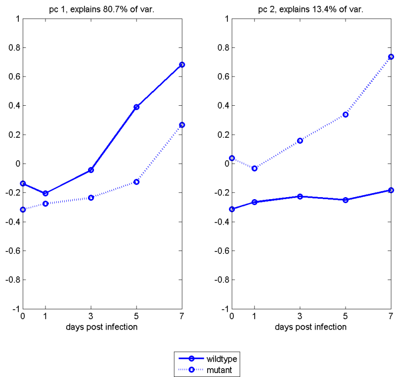
Figure 4. First two principal components of the Arabidopsis powerderly mildew infection experiment.
