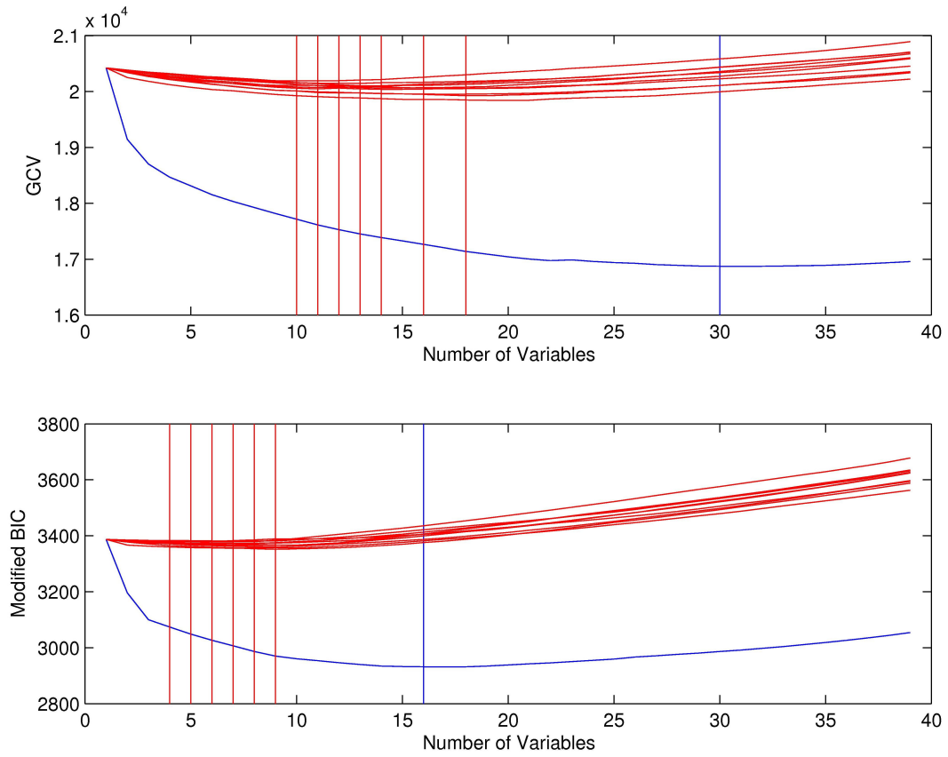
Figure 5. Permutation analysis for Arabidopsis powdery mildew infection data. The top and bottom plots show, respectively, the wGCV and wmBIC curves for 10 randomly decoupled data sets (red lines) versus the real data set (blue line). Vertical lines show the model size that minimizes these curves.
