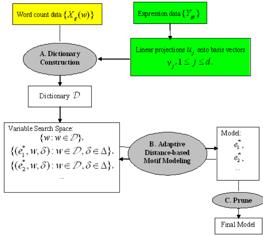
Figure 1. Flow diagram of the analysis process. We start with the multivariate expression data for a filtered set of genes (green boxes) and the counts of all nondegenerate motifs of pre-specified lengths in the upstream promoter sequence of these genes (yellow box). Linear contrasts \mathbf{u}_j of the expression data are used to build the dictionary (step A), and subsequently build the model (step B). The model is then pruned (step C) for parsimony. The steps labeled A,B, and C are detailed in Sections 3.2, 3.3, and 3.4, respectively.
