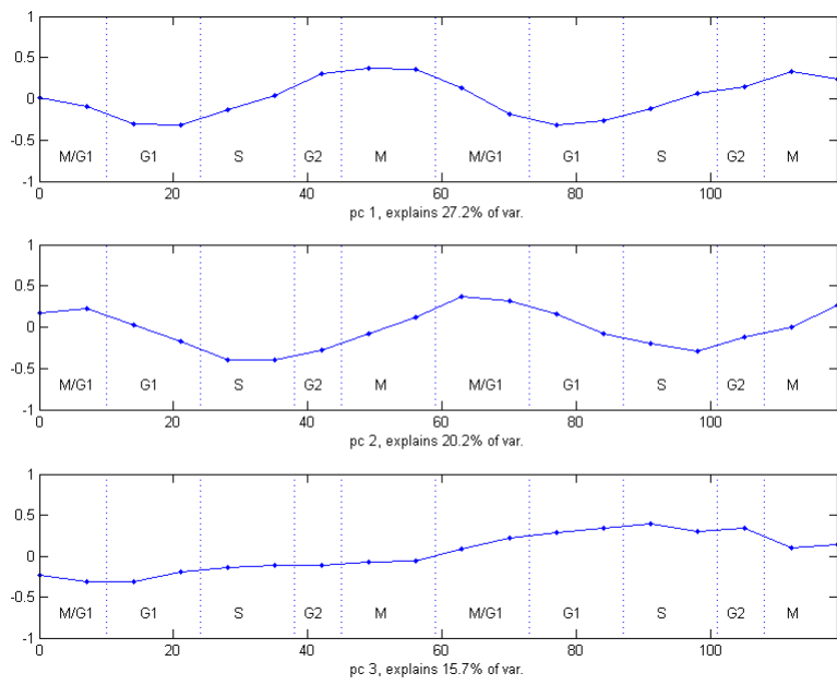
Figure 2. First three principal components of the Spellman et al. (1998) yeast cell cycle experiment.
