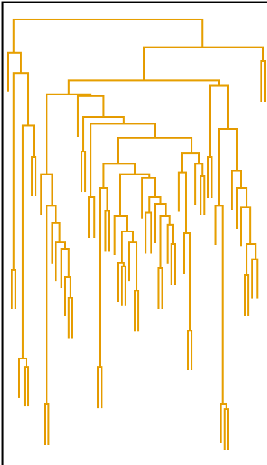
Average Linkage
