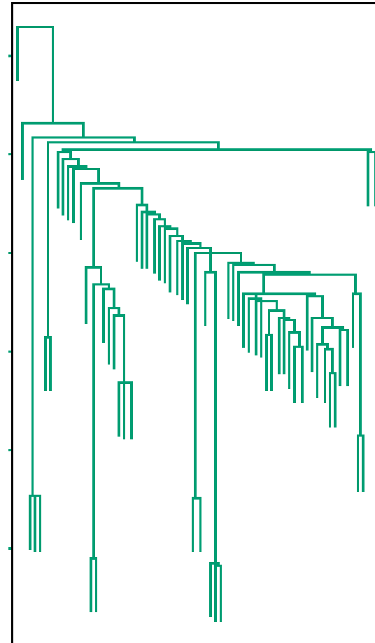
Single Linkage
