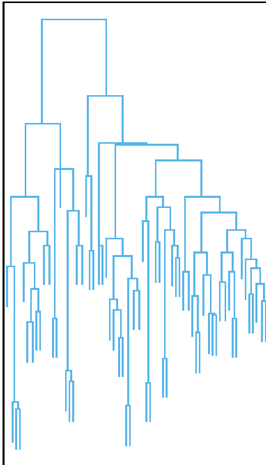
Complete Linkage
