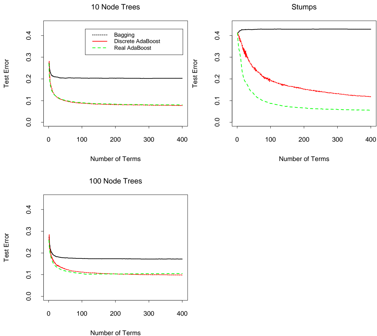
Figure 1: Test error for Bagging, Discrete AdaBoost and Real AdaBoost on a simulated two-class nested spheres problem (see Section 6 on page 20.) There are 2000 training data points in 10 dimensions, and the Bayes error rate is zero. All trees are grown “best-first” without pruning. The left-most iteration corresponds to a single tree.
