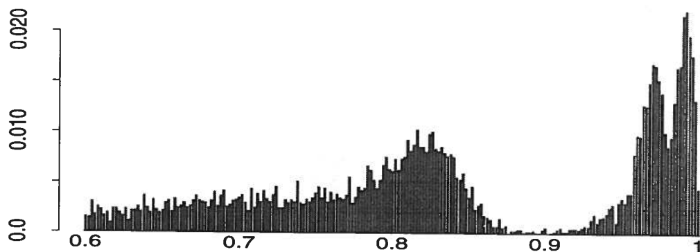
Fig. 4.6. Histogram for Monte Carlo bootstrap: first 10 law school points ( B = 10\,000 )
