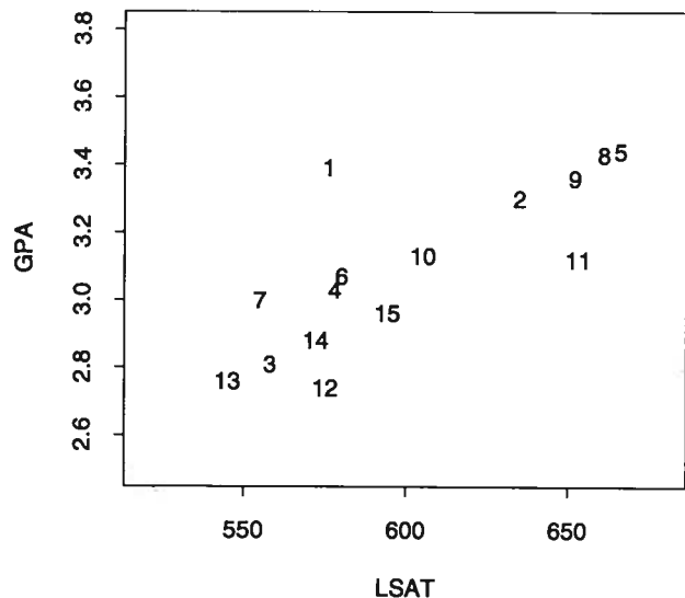
Fig. 4.1. Scatterplot of law school data
