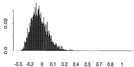
Fig. 4.10. Monte Carlo bootstrap: bioequivalence data, B = 4000
