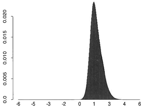
Fig. 4.7. Histogram of \text{arctanh}(\hat{p})
