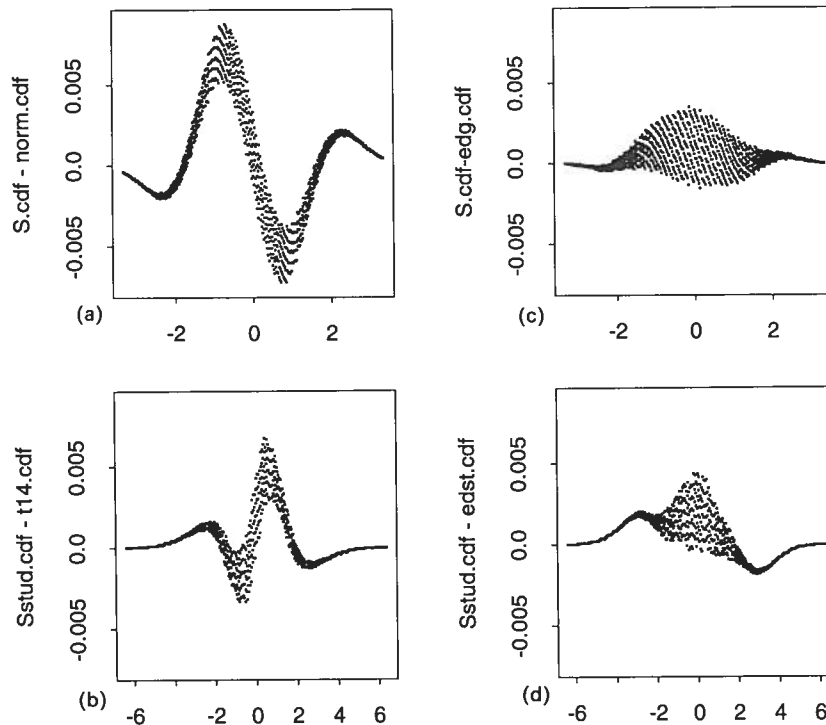
Fig. 2.2. Comparisons between the true and the approximate distributions
