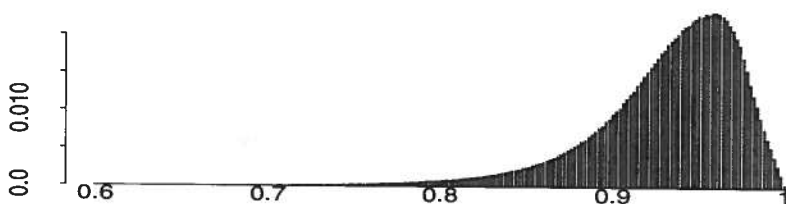
Fig. 4.4. Exhaustive bootstrap without point 1 or 11 (right tail)
