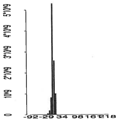
Fig. 2.6. Bootstrap for the median
